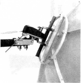
Attach the Dish onto the H-H Motor
